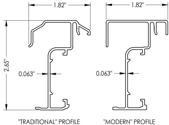
ASTRAGAL SECTIONS
